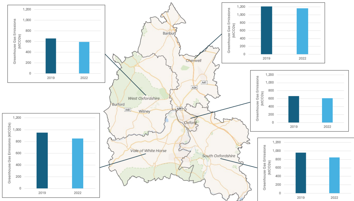
Figure 10: Change in Greenhouse Gas Emissions from 2019 to 2022 by District
