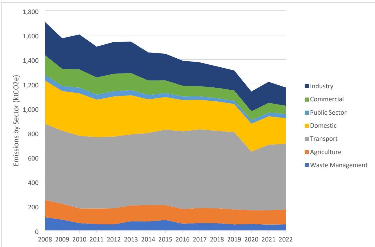
Figure 20: District emissions by sector 2008 - 2022 (Cherwell)
