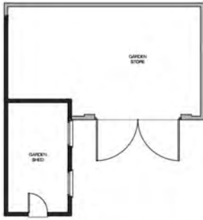
01. PROPOSED GROUND FLOOR PLAN
